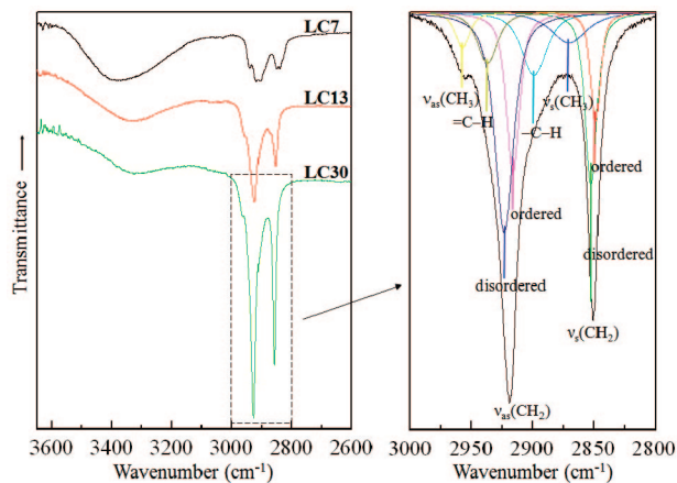
Figure 5. (Left) FTIR spectra of LC7, LC13, and LC30 at room temperature, normalized to the benzene-ring peak at 1605 \text{cm}^{-1} . Values of \nu(\text{OH}) : LC7, \sim 3391 \text{ cm}^{-1} ; LC13, \sim 3321 \text{ cm}^{-1} ; LC30, \sim 3314 \text{ cm}^{-1} . (Right) Deconvolution of the overlapping vibrational bands between 2800 and 3000 \text{cm}^{-1} . Respective values of \nu_{\text{as}}(\text{CH}_2) and \nu_{\text{s}}(\text{CH}_2) : LC7, \sim 2917 and \sim 2848 \text{ cm}^{-1} ; LC13, \sim 2923 and \sim 2853 \text{ cm}^{-1} ; LC30, \sim 2925 and \sim 2857 \text{ cm}^{-1} .
